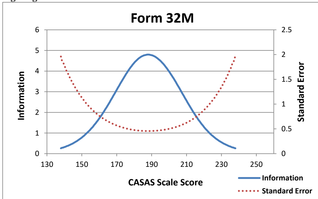
Figure g3-2 Test Information Function – Form 32
