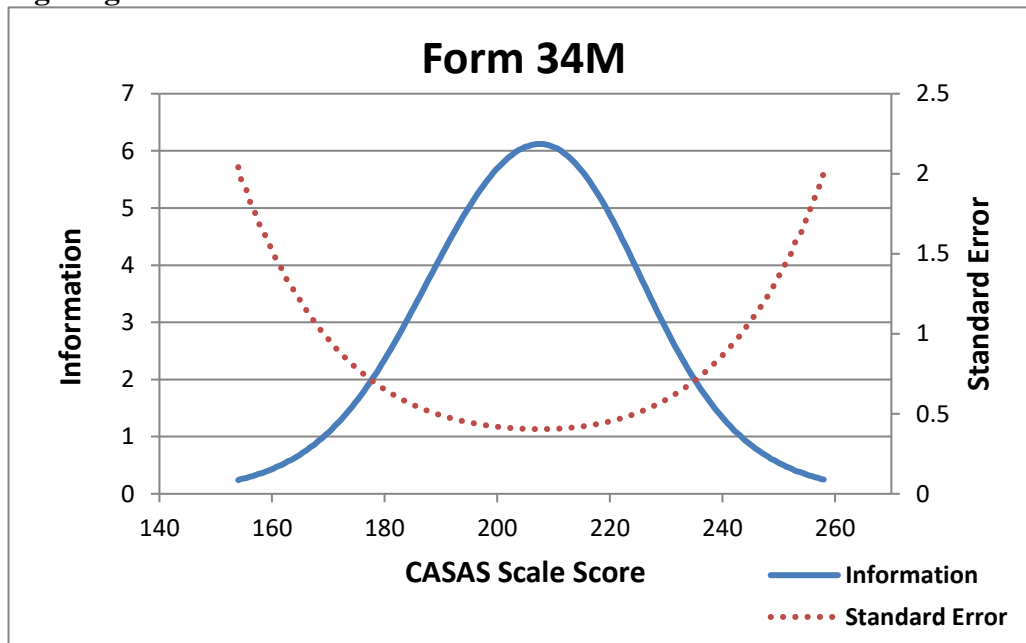
Figure g3-4 Test Information Function – Form 34
